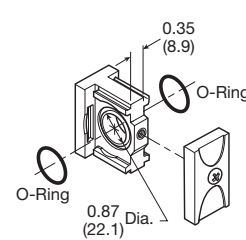
Body Connector
